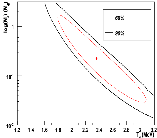
FIG. 4: Two dimensional marginal distribution for accretion parameters M_a and T_a of \bar{\nu}_e with the complete emission model (III C).
