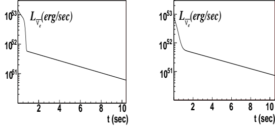
FIG. 6: \bar{\nu}_e luminosity in the LL model (left panel) and in the III C model (right panel).
