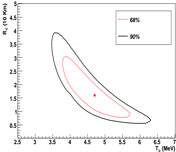
FIG. 3: Two dimensional marginal distribution for cooling parameters R_c and T_c of \bar{\nu}_e with the complete emission model (III C).
