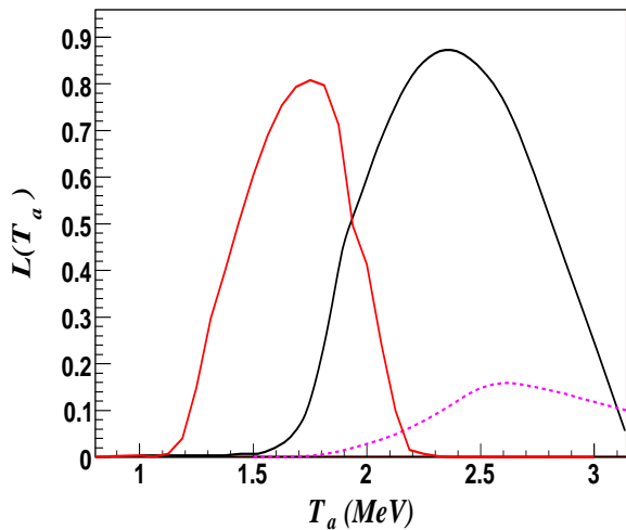
FIG. 2: One dimensional marginal distribution for T_a parameter of accretion with the complete emission model (III.C). The red line is the family of solutions with t_{\text{IMB}}^{\text{off}} \simeq 0.5 . The dark line is the other family of solutions with t^{\text{off}} = 0 and M_a < 1M_\odot . The dotted line is the unphysical family of solutions discussed in Sect. III B \tau_a = 0.2 s.
