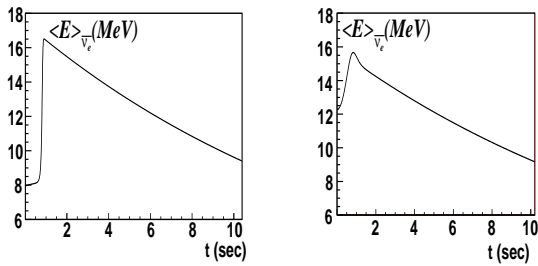
FIG. 5: \bar{\nu}_e mean energy as a function of the time in the LL model (left panel) and in the III C model (right panel).
