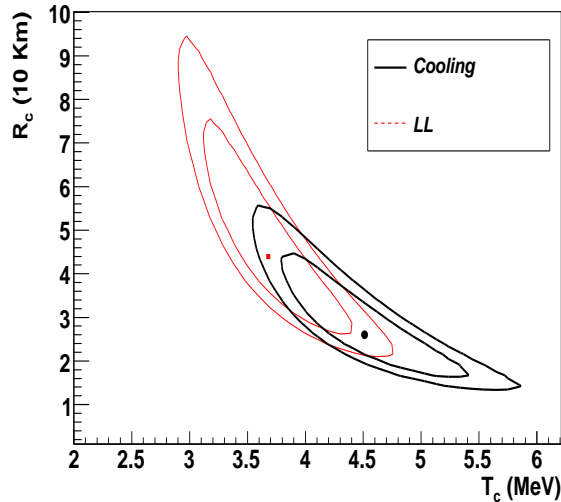
FIG. 1: Two dimensional marginal distributions for the cooling parameters R_c and T_c . The gray (red) contours are the exponential cooling result (68% and 90% C.L.) following Loredo and Lamb analysis. The dark contours are our result for one component cooling model. The best fit points are also displayed.
