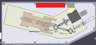
In the picture the accelerator LUNA 400kV and the two different beam lines are visible
