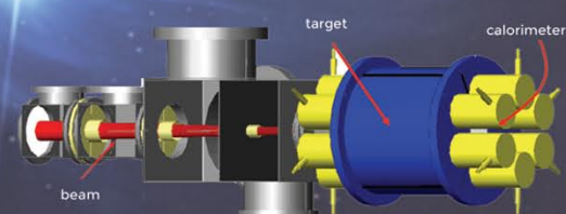
3D reconstruction of the gaseous target
